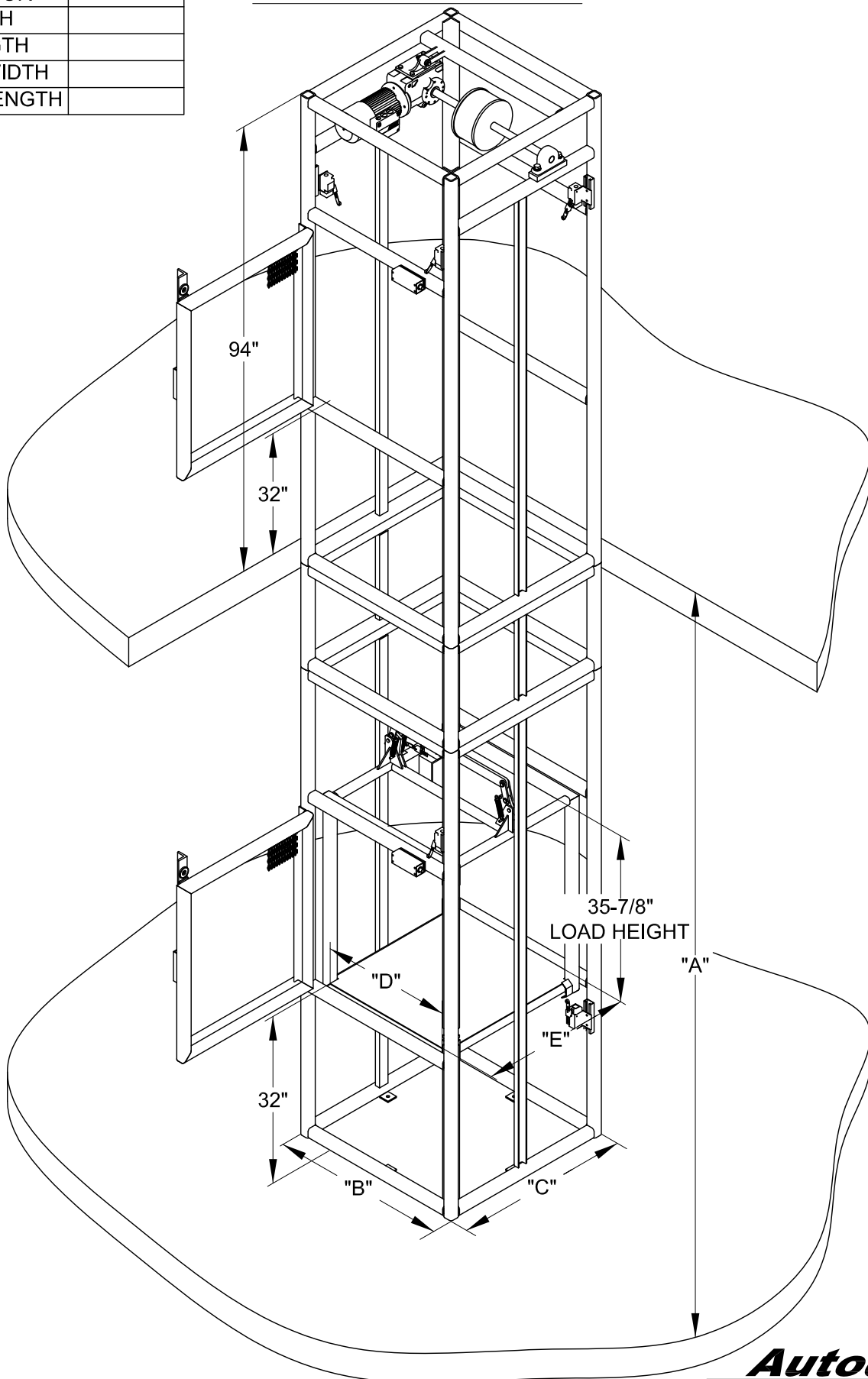
ISOMETRIC VIEW
